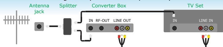
Diagram 1: Use this diagram if you have RCA jacks on your TV.
